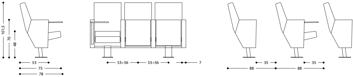
M100 Large su base singola - M100 Large on single base
