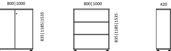
melamine cabinet |armário melamina|armario melamina|armoire melamine
